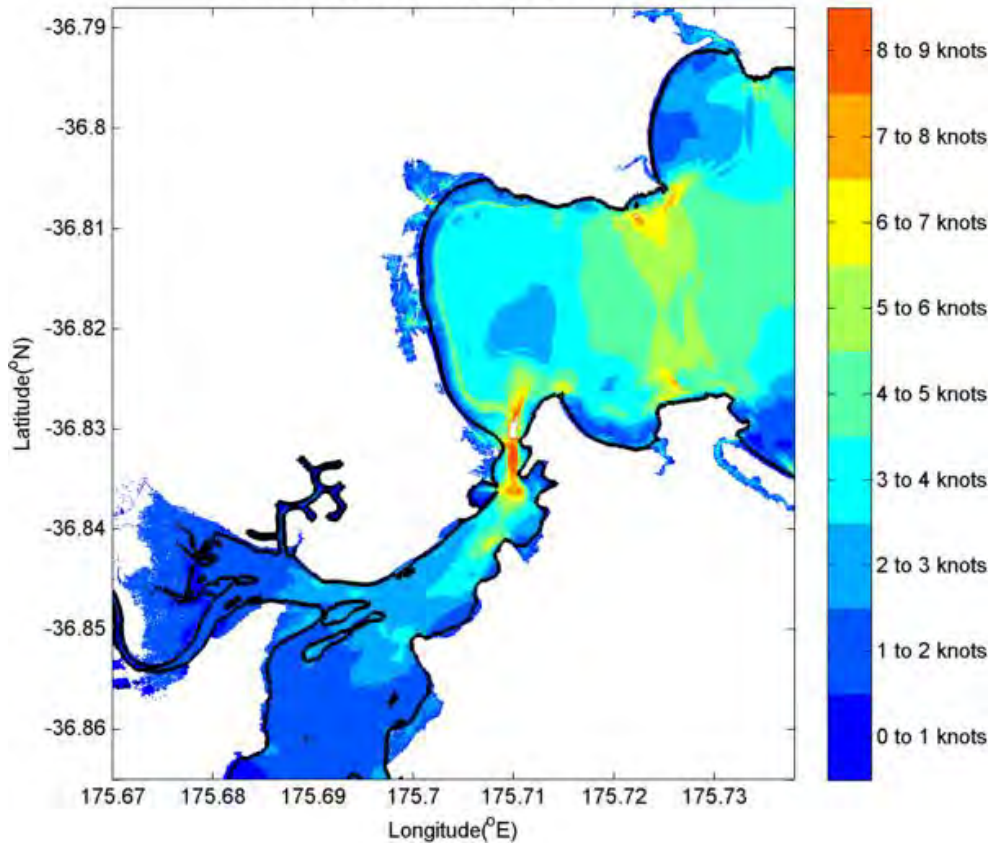
Hazard plot all sources
