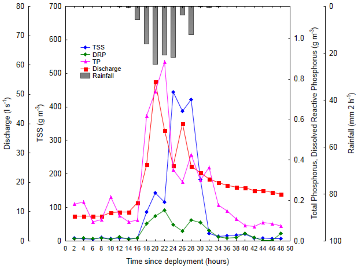
Figure 14. Changes in total phosphorus (TP), dissolved reactive phosphorus (DRP), total suspended solids (TSS), discharge and rainfall at the Rotopiko South 02 monitoring site during the September 2013 storm event. Sampling is at 2 h intervals commencing at 14:20 h on 11 September 2013.
