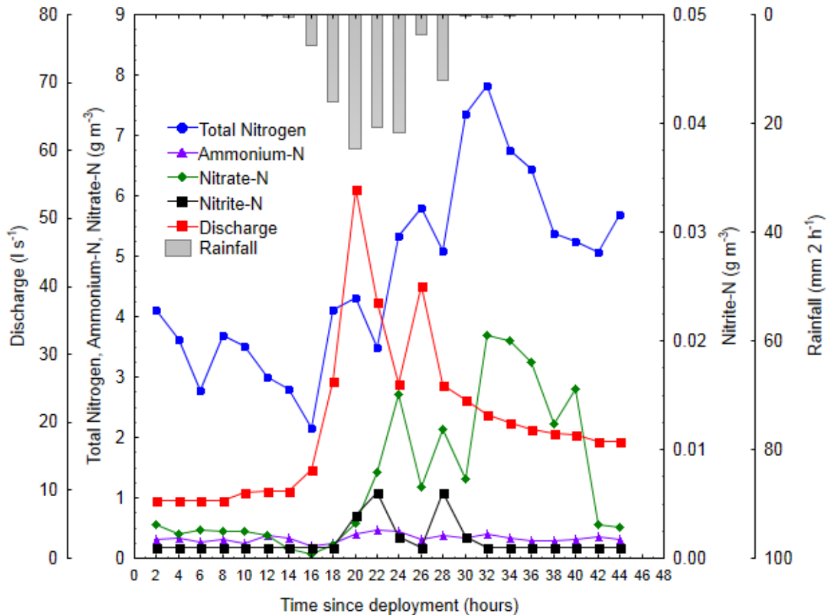
Figure 15. Changes in total nitrogen, ammonium-N, nitrate-N, nitrite-N, discharge and rainfall at the Rotopiko South 02 monitoring site during the September 2013 storm event. Sampling is at 2 h intervals commencing at 14:20 h on 11 September 2013.
