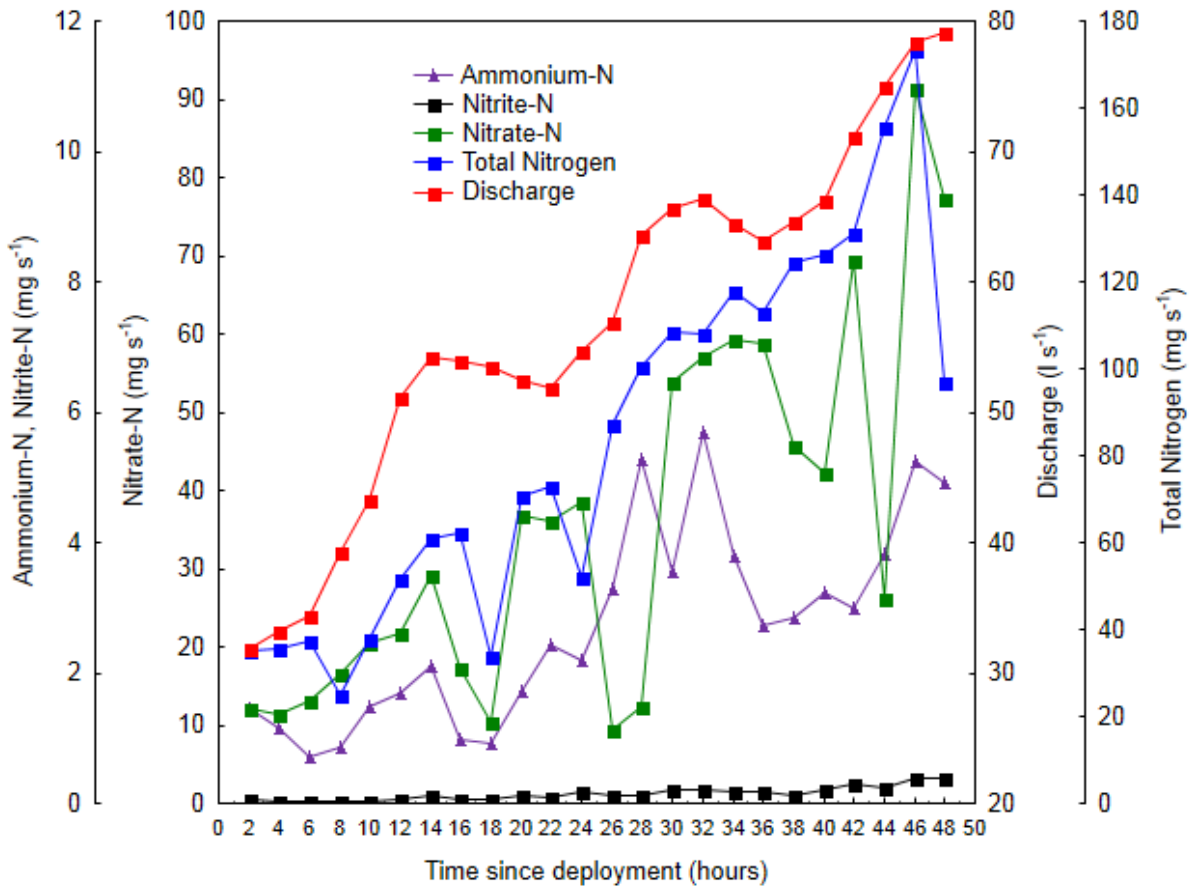
Figure A3.6. Instantaneous total nitrogen, ammonium-N, nitrate-N and nitrite-N loads in relation to discharge for the Mangakaware 06 monitoring site during the 17–19 May 2013 storm event. Sampling is at 2-h intervals commencing at 13:30 h, 17 May 2013.
