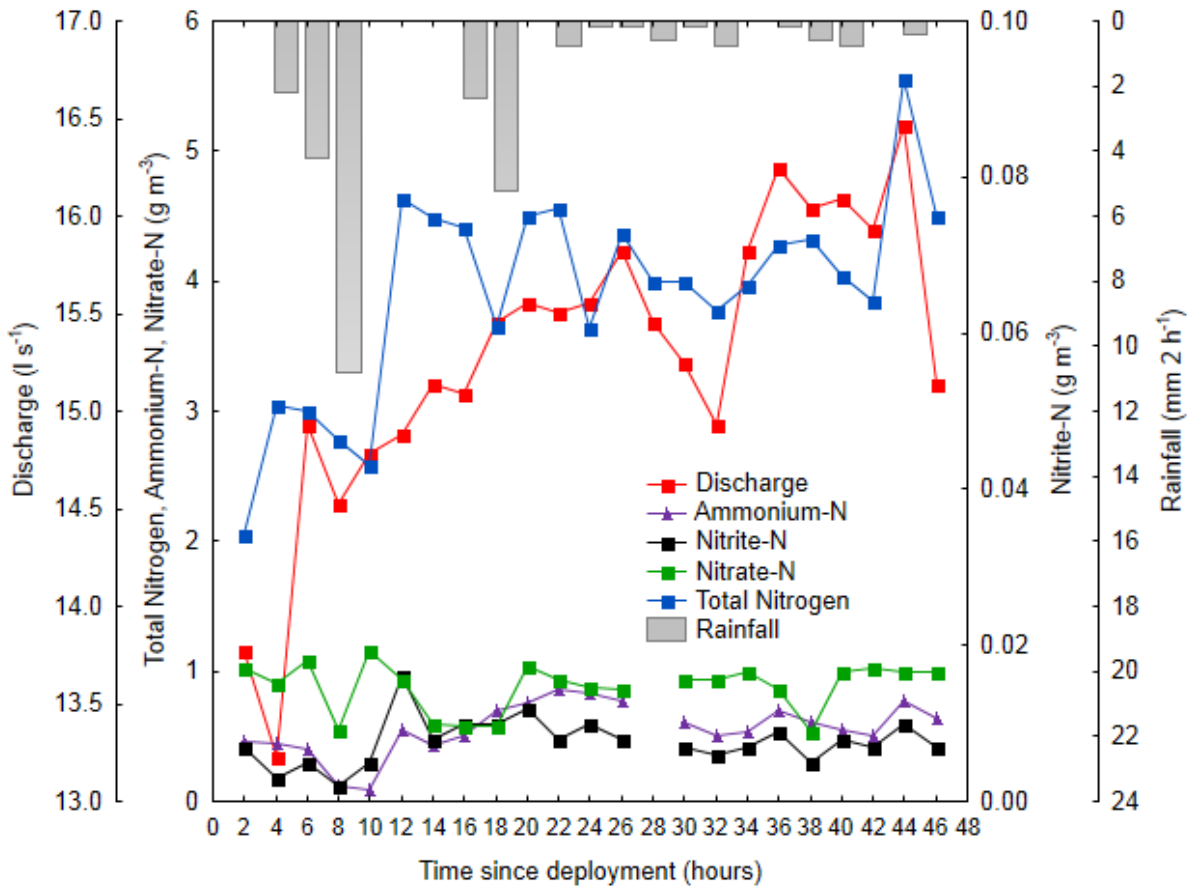
Figure 11. Changes in total nitrogen, ammonium-N, nitrate-N, nitrite-N, discharge and rainfall at the Mangakaware 06 monitoring site during the September 2022 storm event. Sampling is at 2-h intervals beginning at 10:00 h. Note: ammonium-N, nitrate-N and nitrite-N concentrations not available for 28-h sample.
