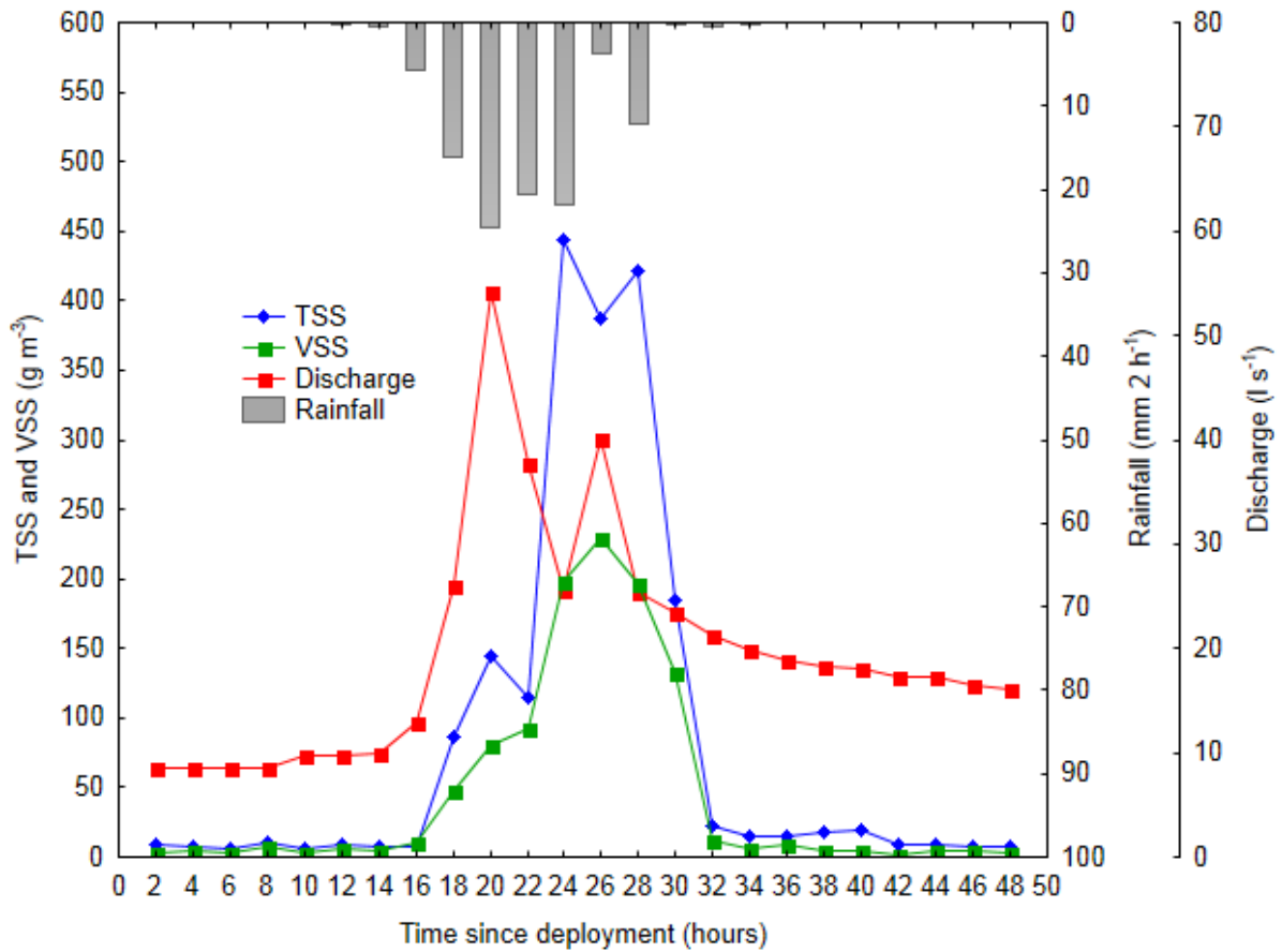
Figure A3.7. Total suspended solids (TSS) and volatile suspended solids (VSS), rainfall and discharge from the Rotopiko South 02 monitoring site for the period 11–13 September 2013. Hour 0 is the time of deployment at 14:20 h on 11 September 2013.
