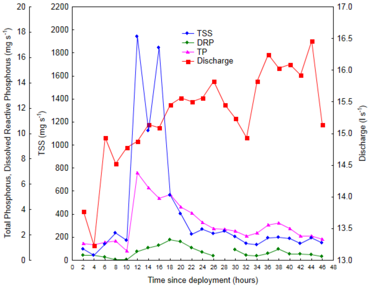
Figure A3.2. Instantaneous total phosphorus (TP), dissolved reactive phosphorus (DRP) and total suspended solids (TSS) loads in relation to discharge for the Mangakaware 06 monitoring site during the September 2012 storm event. Sampling is 2-hourly beginning at 10:00 h. Note: no dissolved reactive phosphorus data available for 28-h sample.
