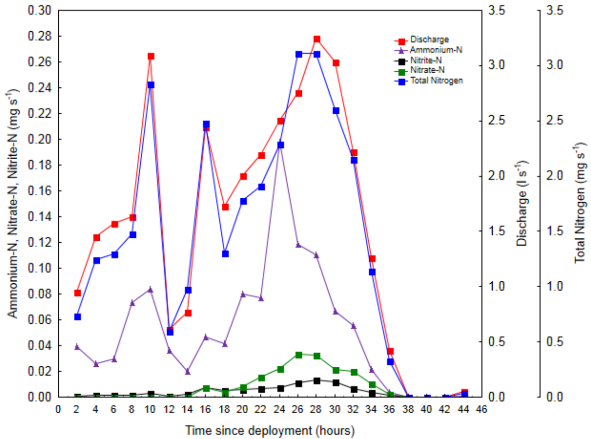
Figure A3.12. Instantaneous total nitrogen, ammonium-N, nitrate-N and nitrite-N loads in relation to discharge for the Mangakaware 05 monitoring site during the January 2014 storm event. Sampling is at 2 h intervals commencing at 11:45 h on 20 January 2014.
