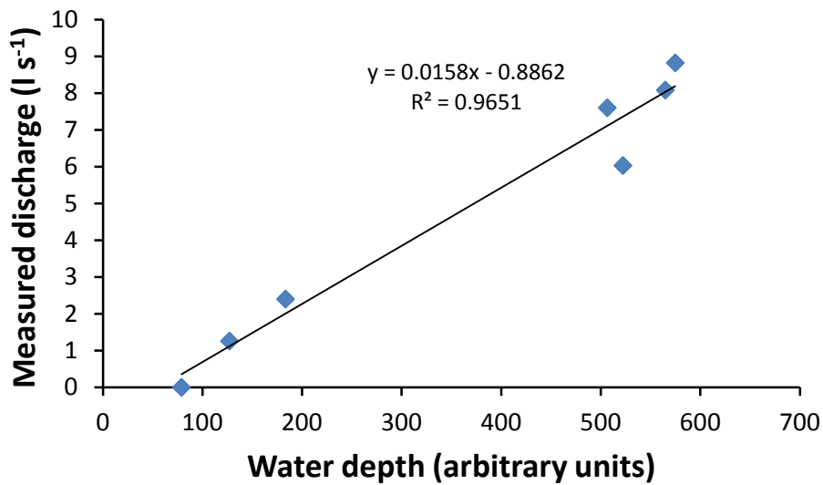
Figure A1.1. Relationship between measured discharge (y) and water depth (x) for the Rotopiko South 02 sampling site. The linear regression equation ( y = 0.0158x - 0.8862 ) derived from this plot was used to calculate discharge from measured water levels.
