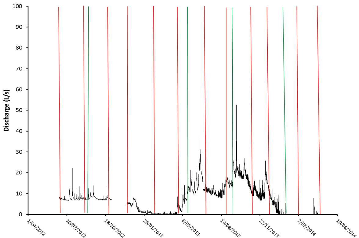
Figure 9. Calculated discharge at Rotopiko South 02 monitoring site from 20 June 2012 to 24 April 2014. Red lines indicate monitoring events; green lines indicate sampled storm events. Due to a fault with the water level logger no data was recorded from 3 November 2012 to 12 December 2012.
