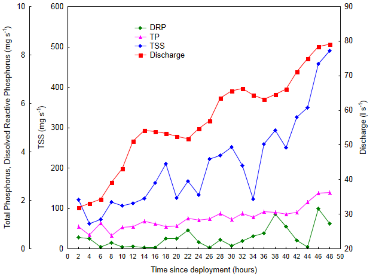
Figure A3.5. Instantaneous total phosphorus (TP), dissolved reactive phosphorus (DRP) and total suspended solids (TSS) loads in relation to discharge for the Mangakaware 05 monitoring site during the 17–19 May 2012 storm event. Sampling is at 2 h intervals commencing at 13:30 h, 17 May 2013.
