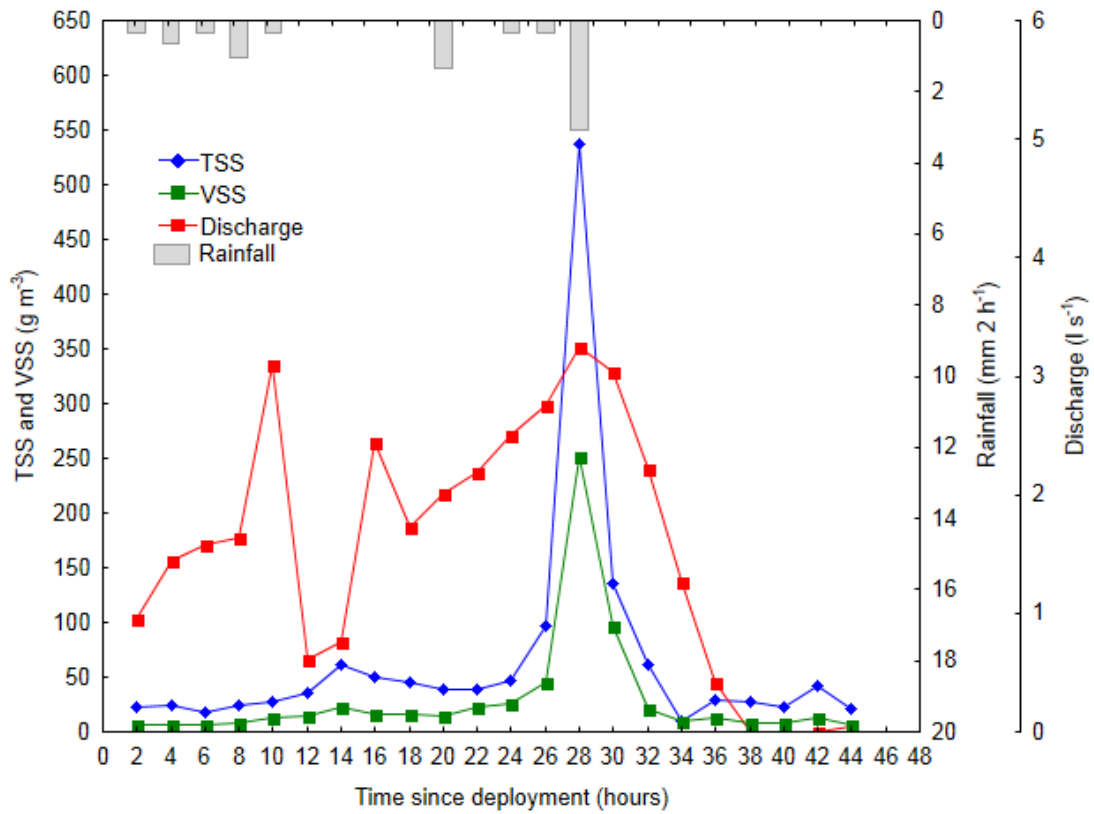
Figure A3.10. Total suspended solids (TSS) and volatile suspended solids (VSS), rainfall and discharge from the Mangakaware 05 monitoring site for the period 20–21 January 2014. Hour 0 is the time of deployment at 11:45 h on 20 January 2014.
