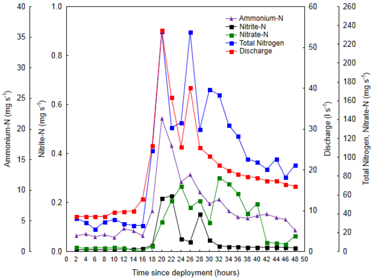
Figure A3.9. Instantaneous total nitrogen, ammonium-N, nitrate-N and nitrite-N loads in relation to discharge for the Rotopiko South 02 monitoring site during the September 2013 storm event. Sampling is at 2 h intervals commencing at 14:20 h on 11 September 2013.
