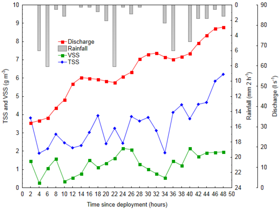
Figure A3.4. Total suspended solids (TSS), volatile suspended solids (VSS), rainfall and discharge from the Mangakaware 05 monitoring site for the period 17–19 May 2013. Hour 0 is the time of deployment at 13:30 h on 17 May 2013.
