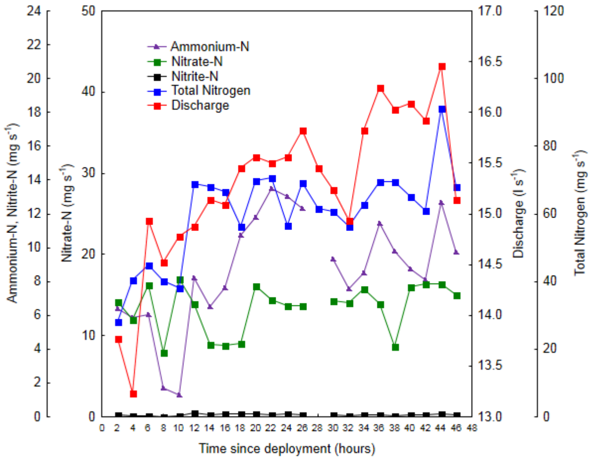
Figure A3.3. Instantaneous total nitrogen, ammonium, nitrate and nitrite loads in relation to discharge for the Mangakaware 06 monitoring site during the September 2012 storm event. Sampling is 2-hourly beginning at 10:00 h. Note: no ammonium-N, nitrate-N and nitrite-N data available for 28-h sample.
