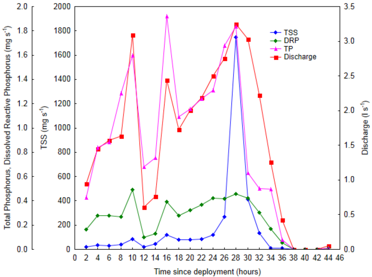
Figure A3.11. Instantaneous total phosphorus (TP), dissolved reactive phosphorus (DRP) and total suspended solids (TSS) loads in relation to discharge for the Mangakaware 05 monitoring site during the January 2014 storm event. Sampling is at 2 h intervals commencing at 11:45 h on 20 January 2014.
