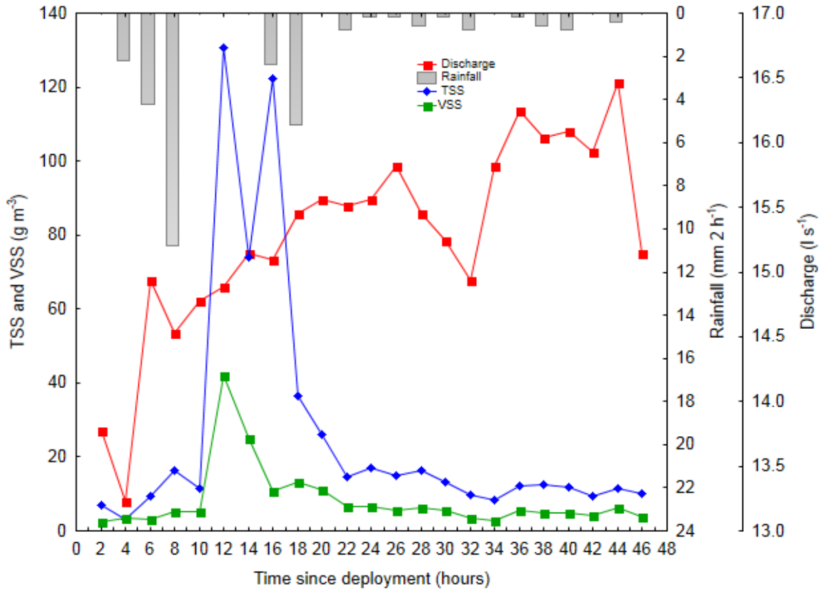
Figure A3.1. Total suspended solids (TSS) and volatile suspended solids (VSS) from the Mangakaware 06 monitoring site for the period 3–5 September 2012. Two-hour rainfall data sourced from NIWA National Climate Database, Hamilton Airport station (12 km). Discharge calculated from water level height is also presented. Hour 0 is the time of sampler deployment at 10:00 h on 3 September 2012.
