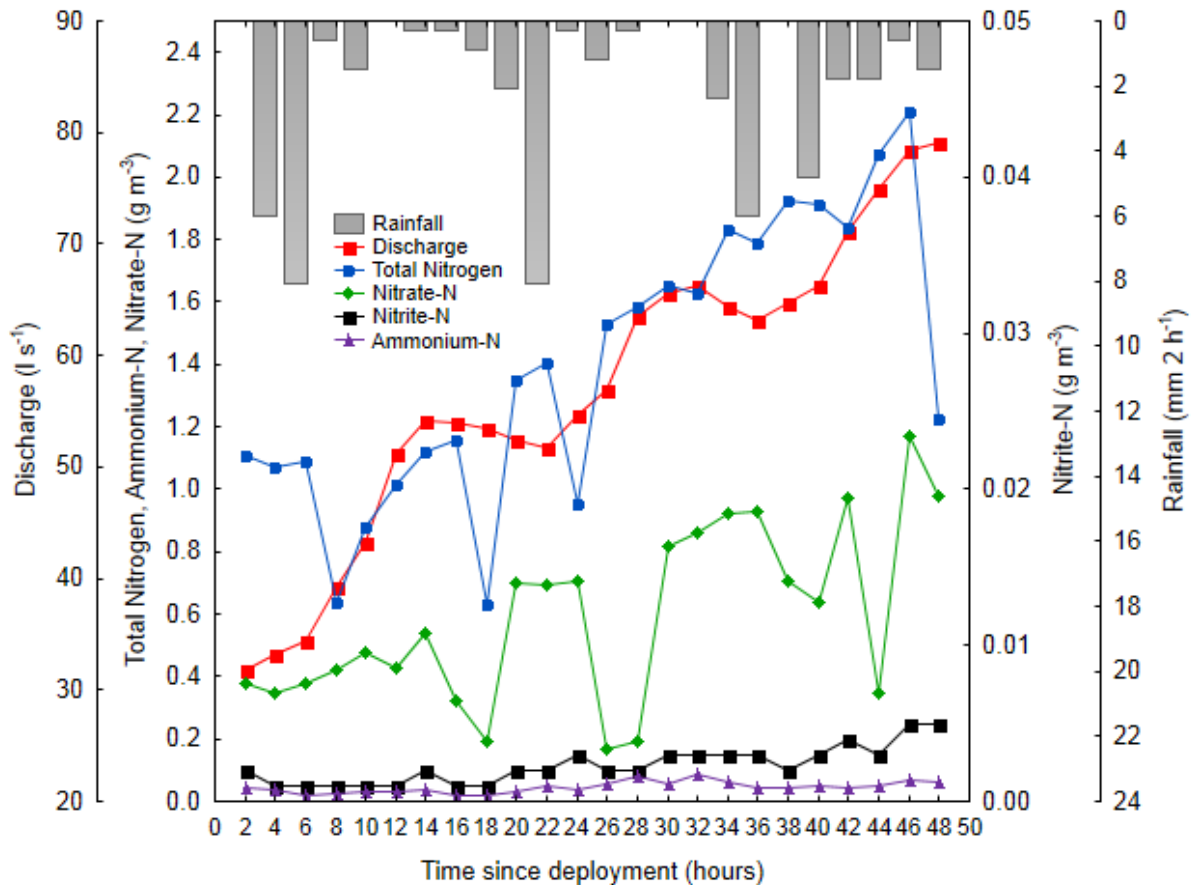
Figure 13. Changes in total nitrogen, ammonium-N, nitrate-N, nitrite-N, discharge and rainfall at the Mangakaware 05 monitoring site during the 17-19 May 2013 storm event. Sampling is at 2 h intervals commencing at 13:30 h, 17 May 2013.
