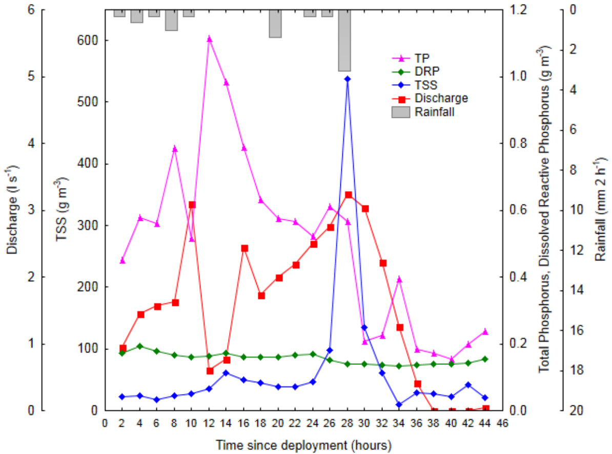
Figure 16. Changes in total phosphorus (TP), dissolved reactive phosphorus (DRP), total suspended solids (TSS), discharge and rainfall at the Mangakaware 05 monitoring site during the January 2014 storm event. Sampling is at 2 h intervals commencing at 11:45 h on 20 January 2014.
