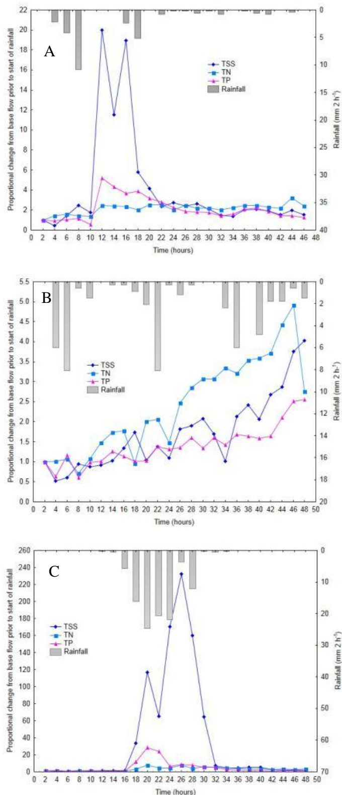
Figure 18. Proportional changes in TSS, TN and TP in relation to base flow concentrations for A) Mangakaware 06 (September 2012), B) Mangakaware 05 (May 2013) and C) Rotopiko South 02 (September 2013). Data for the Mangakaware 05 inflow (January 2014) are omitted as there was no measureable discharge prior to the commencement of rainfall.
