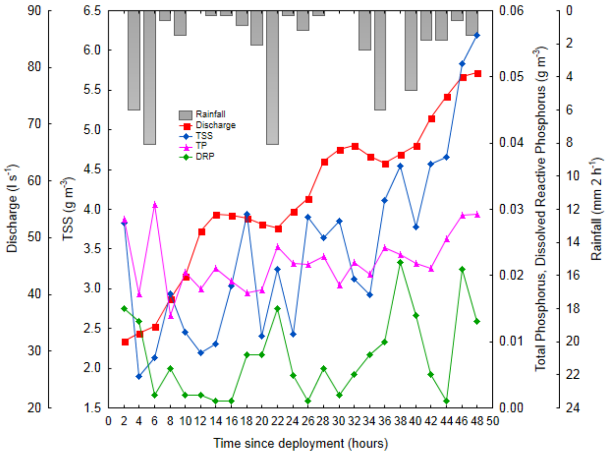
Figure 12. Changes in total phosphorus (TP), dissolved reactive phosphorus (DRP), discharge, total suspended solids (TSS) and rainfall at the Mangakaware 05 monitoring site during the 17-19 May 2013 storm event. Sampling is at 2 h intervals commencing at 13:30 h, 17 May 2013.
