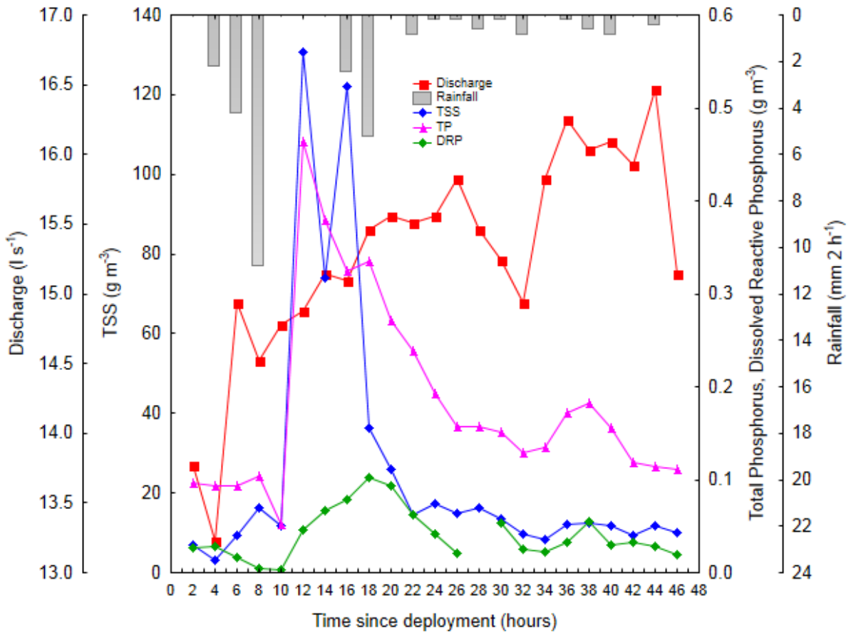
Figure 10. Changes in total phosphorus (TP), dissolved reactive phosphorus (DRP), discharge, total suspended solids (TSS) and rainfall at the Mangakaware 06 monitoring site during the September 2012 storm event. Sampling is at 2-h intervals beginning at 10:00 h. Note: dissolved reactive phosphorus sample not available for 28-h due to sample container leakage.
