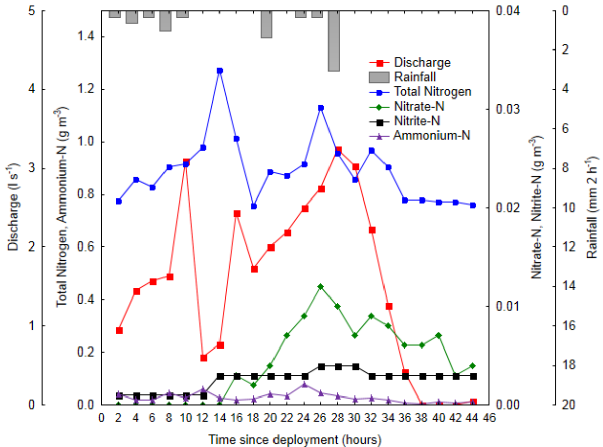
Figure 17. Changes in total nitrogen, ammonium-N, nitrate-N, nitrite-N, discharge and rainfall at the Mangakaware 05 monitoring site during the January 2014 storm event. Sampling is at 2 h intervals commencing at 11:45 h on 20 January 2014.
