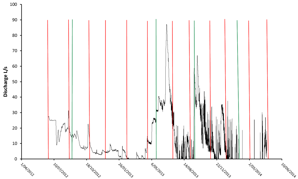
Figure 8. Calculated discharge at Mangakaware 06 monitoring site from 20 June 2012 to 24 April 2014. Red lines indicate monitoring events; green lines indicate sampled storm events.
