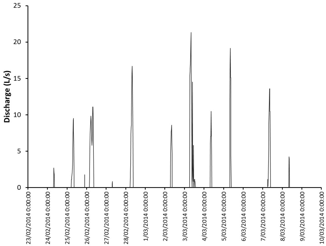
Figure 7. Example of the periodic discharge observed at the Mangakaware 05 monitoring site during late summer and early autumn of 2014. Discharge typically commenced at 05:00 h and ended by 10:00 h.
