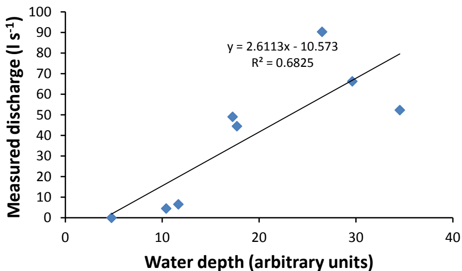
Figure A1.2. Relationship between measured discharge (y) and water depth (x) for the Mangakaware 05 sampling site. The linear regression equation ( y = 2.6113x - 10.573 ) derived from this plot was used to calculate discharge from measured water levels.
