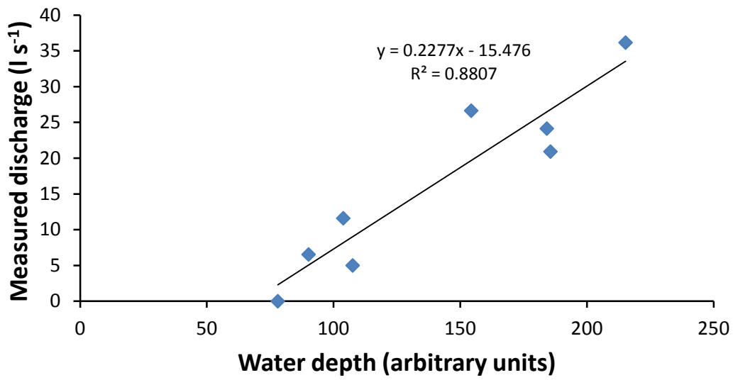
Figure A1.3. Relationship between measured discharge (y) and water depth (x) for the Mangakaware 06 sampling site. The linear regression equation ( y = 0.2277x - 15.476 ) derived from this plot was used to calculate discharge from measured water levels.
