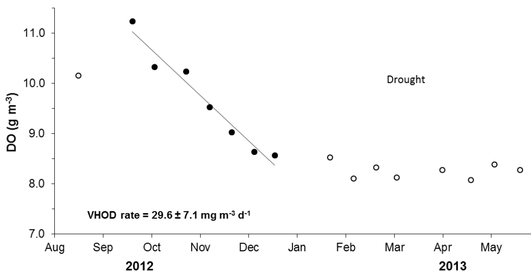
Figure 7: VHOD for 2012-2013 monitoring period. Volume-weighted mean dissolved oxygen (DO) concentrations below 70 m for 2012/13. The slope of the linear regression through the solid data points provides the VHOD rate. ( P < 0.0001 , r^2 = 0.96 , n = 7 ). Data from January 2013 on show little change indicating re-oxygenation was occurring, balancing sediment oxygen demand.
