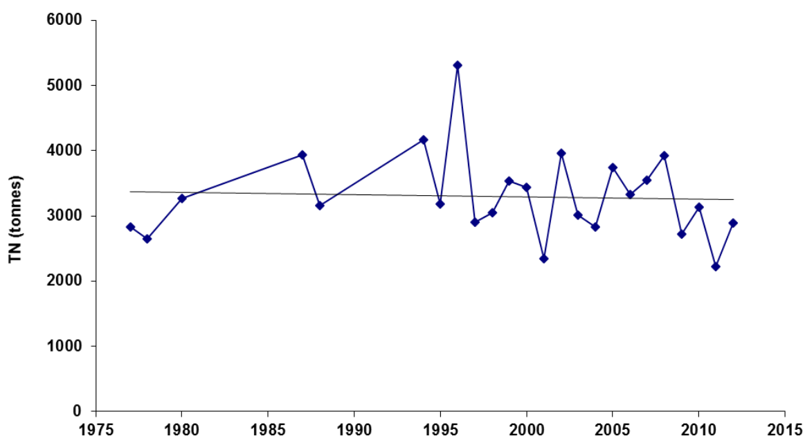
Figure 22: Estimates of the mass of total nitrogen (TN) in Lake Taupo. Although there was an average decrease of about 3.8 \text{ t y}^{-1} from 1975 to 2013, this apparent trend in the data is not statistically significant ( P = 0.79 , n=24 , r^2 = 0.003 ). The mean was 3294 t. Date ticks are 1 January in each year.
