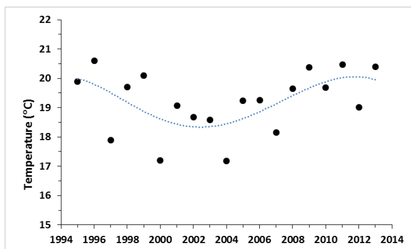
Figure 3: Maximum 20 m temperatures in summer. The trend line is a 5th order polynomial indicating a cyclical pattern.
