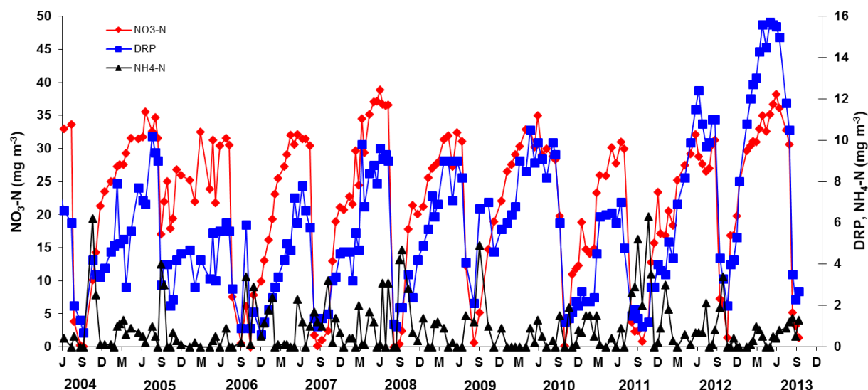
Figure 18: Time series bottom water nutrient data. \text{DRP} , \text{NO}_3\text{-N} and \text{NH}_4\text{-N} concentrations in the bottom waters (150 m depth) of Lake Taupo since winter mixing of 2004. (Starting tick “J” = June with 3-monthly increments).
