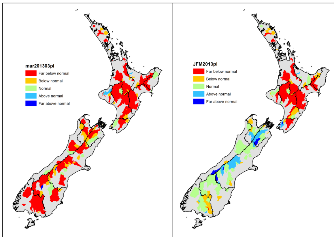
Figure 4: NIWA soil moisture anomaly maps for March 2013 (left) and the period from January to March 2013 (right) showing the extent of the drought. The whole of the Lake Taupo catchment was affected for at least three months.
