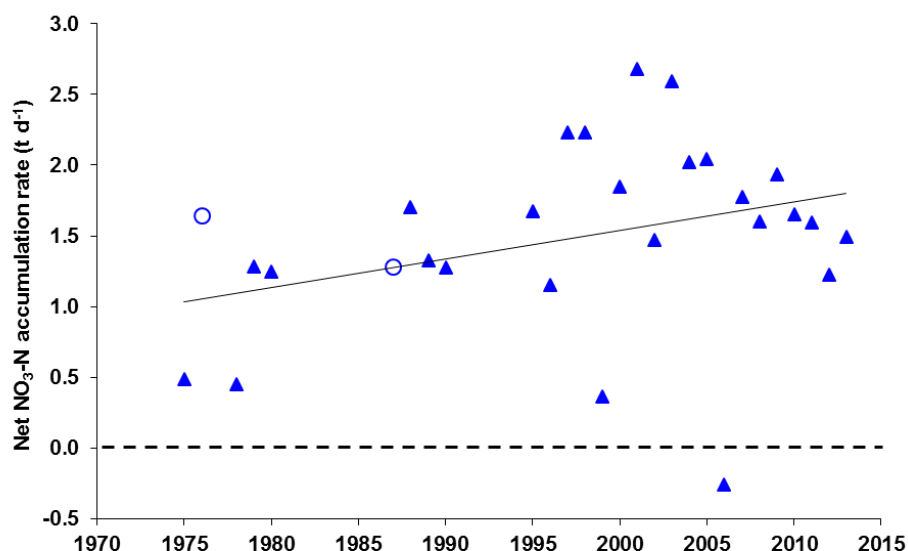
Figure 21: Net Hypolimnetic \text{NO}_3\text{-N} accumulation rates. Net \text{NO}_3\text{-N} accumulation rates ( \text{t d}^{-1} ) in the hypolimnion below 70 m. The regression line shows an increase in the net accumulation rate of 0.020 \pm 0.024 \text{t d}^{-1} ( P = 0.1 , r^2 = 0.15 , n = 26 ). Open circle data were not included in the regression analysis (see text). Note that the Y-axis extends to -0.5 \text{t d}^{-1} for the 2006 data point. Date ticks are 1 January in each year.
