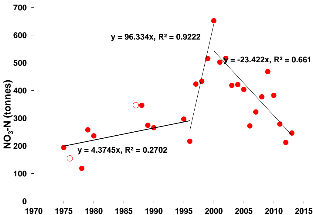
Figure 20: Changes in nitrate (NO 3 -N) accumulation in the hypolimnion of Lake Taupo. The last regression line shows that in the last 14 years, NO 3 -N mass has decreased at a significant average rate of around 23 \text{ t y}^{-1} ( P < 0.001 , r^2 = 0.66 , n = 14 ) and is now comparable with the estimated mass present in the late 1970s and early 1980s.
