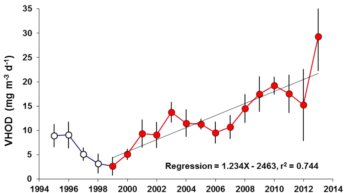
Figure 8: Time-series VHOD data. Time-series of VHOD rates since 1994-5. The low VHOD in 1997-2000 (following the 1995/96 eruptions of Mount Ruapehu) correlates with a shift in algal dominance from diatoms to colonial greens ( Botryococcus braunii ). The regression through the solid (red) dots ( P < 0.0001 , r^2 = 0.74 , n = 15 ), only refers to the change in VHOD since 1998/99, the year when the VHOD rate during the monitoring programme was lowest, and the last year in which diatoms were not dominant. Bars are SD.
