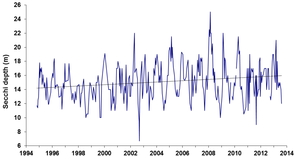
Figure 9: Water clarity as measured by Secchi depth. Time-series Secchi depth data for the present monitoring programme since 1994. Trend line equation 0.060 \pm 0.051 \text{ m y}^{-1} ( P = 0.02 , r^2 = 0.016 n = 332 ) based on daily data.
