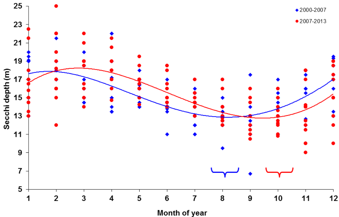
Figure 11: The timing of minimum water clarity has recently changed. Between 2000 and 2007 (blue), minimum water clarity occurred in winter (August). Since 2007 (red) minimum water clarity has occurred two months later in spring (October). Water clarity in summer was higher after 2007 than before. Curves are 4 th order polynomials fitted to the data.
