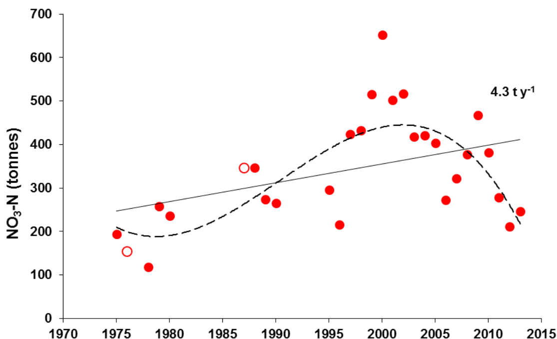
Figure 19: Total mass of \text{NO}_3\text{-N} in the hypolimnion of Lake Taupo in autumn before winter mixing. The linear regression (solid line) indicates a statistically significant increase of 4.3\text{ t y}^{-1} ( P < 0.05 , r^2 = 0.15 , n = 26 ). Temporal changes in the data are better described by a 3 rd order polynomial (dashed line) ( r^2 = 0.556 ) which accommodates a rise and fall in the data over the monitoring period since 1974. Open circle data were excluded from regression as time periods and sampled depths were not the same as used for the other data. Date ticks are 1 January in each year.
