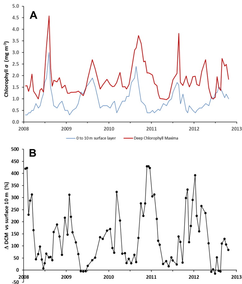
Figure 15: DCM data from 2008 to 2012. A) Comparison of chlorophyll a concentrations in the 0 to 10 m layer and the chlorophyll a in the DCM layer calculated from calibrated chlorophyll fluorescence profiles, and B) The difference between the DCM and the 0 to 10 m depth layer, as a percentage of the surface concentration.
