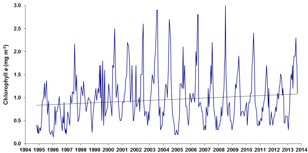
Figure 12: Time-series chlorophyll a concentrations in the upper 10 m of Lake Taupo. The solid regression line represents a statistically significant increase in the mean chlorophyll a concentrations of 0.013 \pm 0.0107 \text{ mg m}^{-3} \text{ y}^{-1} ( P = 0.016 , r^2 = 0.0175 , n = 331 ). Date ticks are 1 January in each year.
