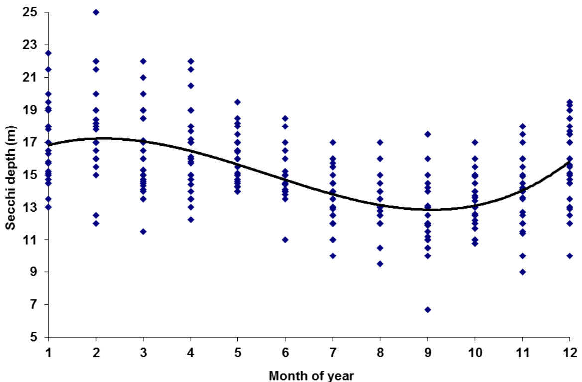
Figure 10: Seasonal cycle of water clarity (1994 -2013). The annual pattern of all water clarity data has a seasonal cycle with minimum clarity occurring usually in September.
