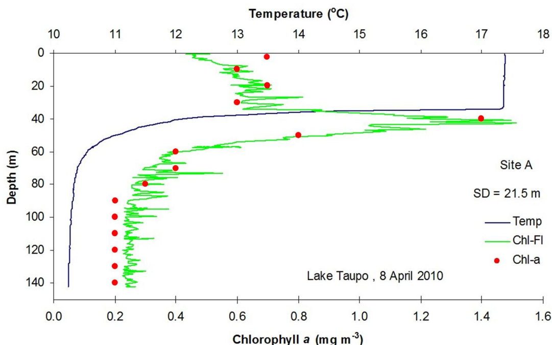
Figure 14: Deep chlorophyll maxima. Example of a deep chlorophyll maxima in Lake Taupo measured by chlorophyll fluorescence (Chl-FI) on 8 April 2010 compared with extracted chlorophyll a (Chl- a ) concentrations (red dots) from water samples collected at 10 m depth intervals on the same day. The peak phytoplankton biomass lies just below the thermocline.
