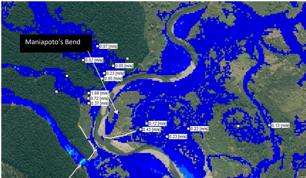
Figure App B1: Velocity at Maniapoto's Bend 10% AEP
