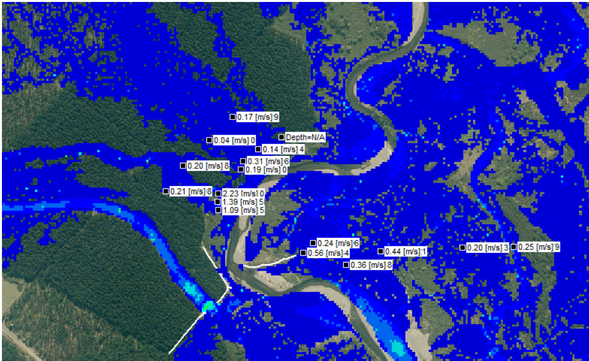
Figure App B3: Velocity at Maniapoto's Bend 2% AEP
