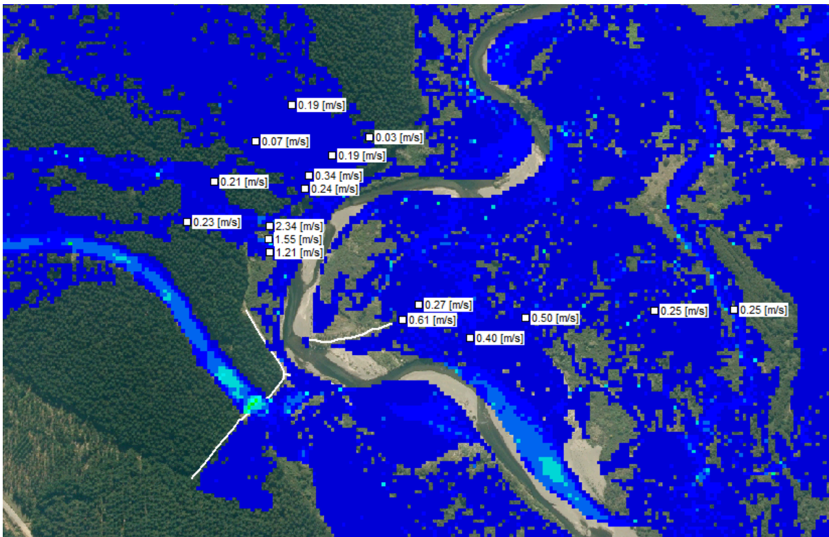
Figure App B4: Velocity at Maniapoto's Bend 1% AEP
