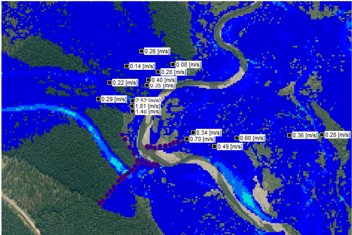
Figure App B5: Velocity at Maniapoto's Bend 1% AEP plus climate change
