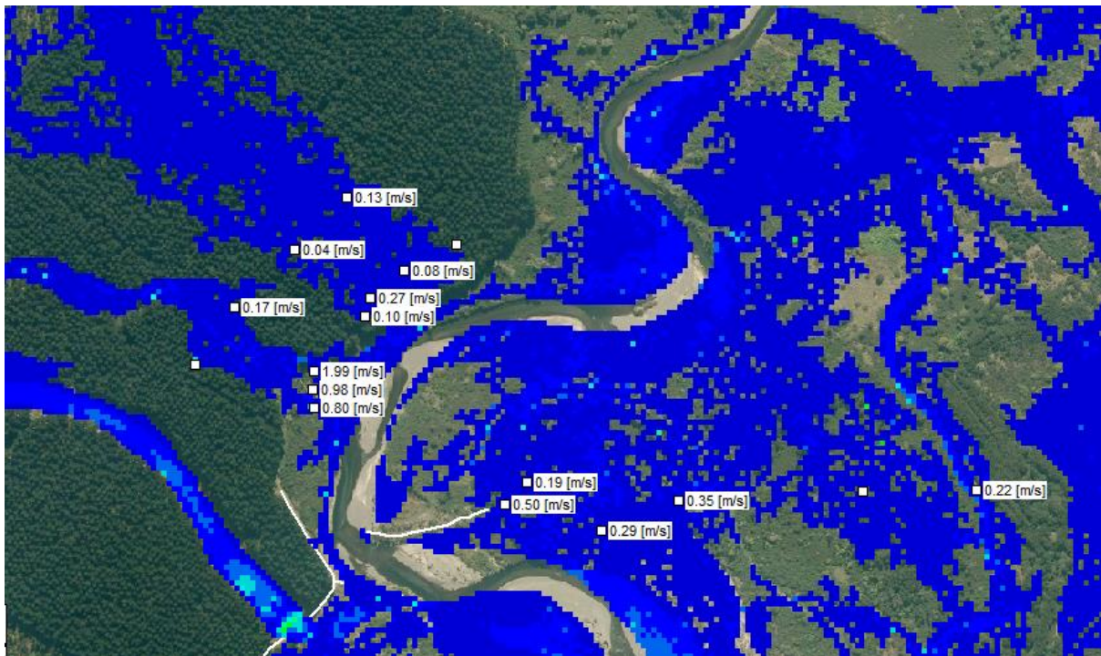
Figure App B2: Velocity at Maniapoto's Bend 5% AEP
